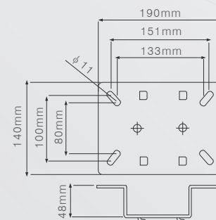
Mounting bracket dimensions
